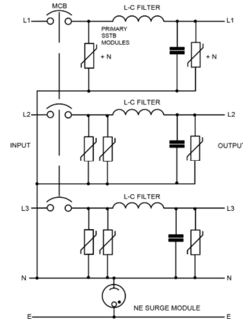
Schematic of 3 Ø surge filter
