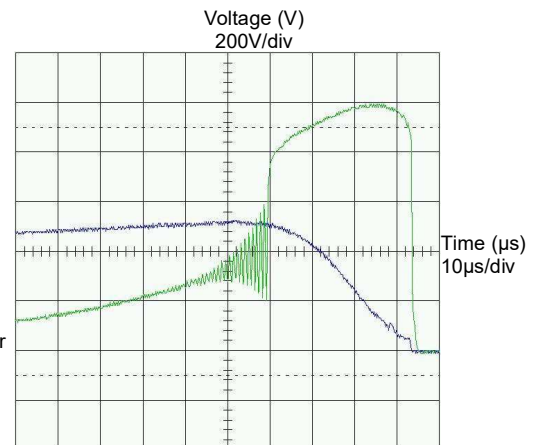
Green: Shunt Protector Blue: Series Filter
